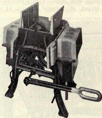
FIG. 13—DOUBLE-SIDED FACE-DOWN BLOCK MACHINE Cores are withdrawn downward after block has been turned over
